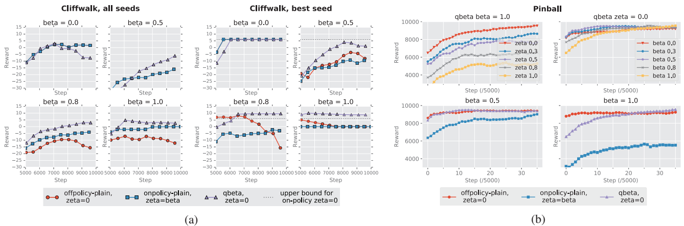
Figure 3: Control performance. (a) Cliffwalk. Each variant is evaluated on 5 seeds for 10 runs each. Left : Average performance per value of \beta on all seeds. Right : Learning curves for the best seeds per variant. Notice how Q(\beta) is the only variant that escapes the plateau of the suboptimal policy. (b) Pinball. Each variant is evaluated on 20 independent runs. Top row : Influence of \beta and \zeta on Q(\beta) : performance improves as \zeta gets smaller. Overall, intermediate target \beta -s are best, but \beta = 1 reaches slightly better performance at the end of learning. Bottom row : Comparison within the variants for select values of \beta
