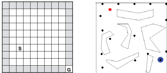
Figure 4: Left : The modified cliffwalk task. Shaded regions are cliffs. Right : Pinball domain configuration used. The red ball must be moved to the blue hole. Each black diamond indicates an option landmark.
