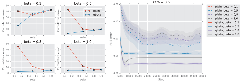
Figure 1: Prediction error on the 19-state chain task. Each variant is an average of 10 seeds. Left : Sum error for each \zeta - \beta combination. Q(\beta) always gets more efficient as \zeta decreases (the options get longer). Right : Example learning curves. The lines corresponding to \beta = 0.1 are outside the axes’ bounds. The shaded region covers standard deviation.
