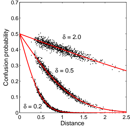
Fig. .1. The probability of confusion as a function of distance for several values of \delta . The curves give the theoretical prediction based on the calculations in section 3.2; the points are data from a computational simulation of the confusion probabilities between two trajectories in a 2d acoustic space (discussed in section 3.4).
