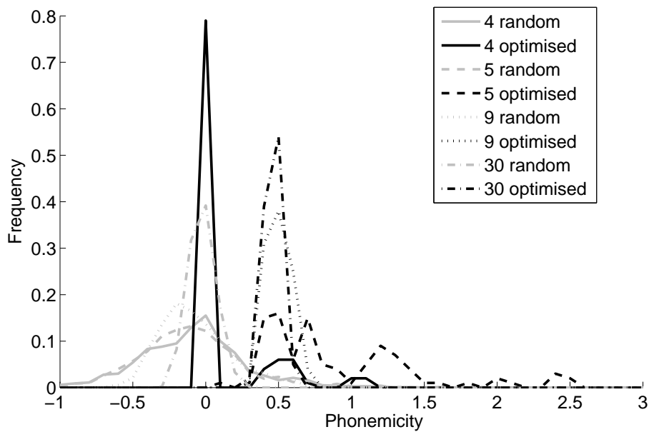
Fig. .13. Optimised repertoires always show a significantly higher degree of phonemicity (as defined in the appendix) than random repertoires. Shown are the frequencies (y-axis) with which a certain degree of phonemicity (x-axis) is obtained in 100 runs for each condition. Conditions varied in the number of trajectories per repertoire (4, 5, 9 and 30) and whether or they were randomly chosen or optimised (the OP criterion from section 3.5). For all repertoire sizes larger than four, the differences between the random and optimised conditions are highly significant.
