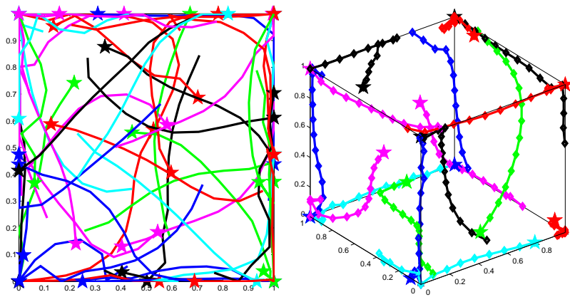
(a) 2d example with many trajectories optimized for distinctiveness. T = 50, P = 10, \rho = 0.2, S = 0.1, \delta = 0.1, I = 5000 .
