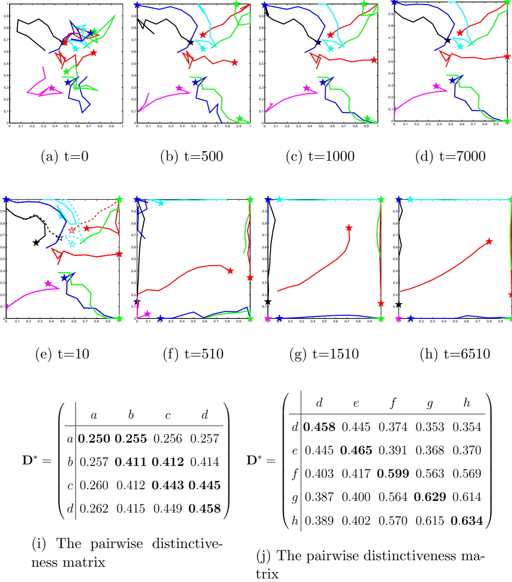
Fig. 10. Locally optimal repertoires are ESSs, but not all ESSs are locally optimal. (a-d) show configurations in an evolutionary simulation with the hearer benefit condition (HB, D(R, R') > D(R, R) ) at various time steps; (d) is an ESS in the HB condition; (e-h) show results from a simulation in the optimization condition (OP, D(R', R') > D(R, R) ) that used (d) as its initial condition. (h) is an ESS in all conditions (OP, HB, SB, EB) considered. (i) shows a matrix that gives the pairwise distinctiveness scores for every combination of configurations in (a-d); (j) the matrix that gives the pairwise distinctiveness scores for every combination of configurations in (d-h). The approximate evolutionary trajectory is indicated with bold-face in these matrices. Parameters are: T=9 , P=10 , D=2 , N=0.05 , S=0.1 .
