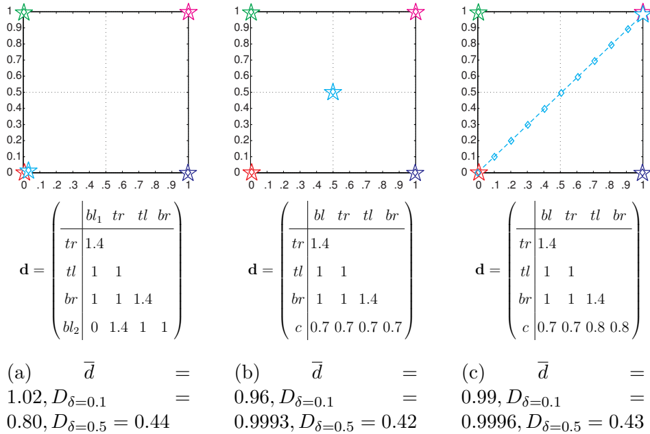
Fig. .7. Why do trajectories stretch out? Three configurations and their distance matrices. Abbreviations: bl : bottom-left, tr : top-right, tl : top-left, br : bottom-right, c center.
