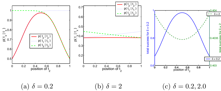
Fig. .4. Distinctiveness as dependent on distance and noise, 1d example. Panel a) shows confusion probabilities in a low-noise environment, panel b) shows them in a high-noise environment. Panel c) compares the probabilities of correct recognition for the low-noise and the high noise conditions. Note that the high-noise condition has a minimum at maximal distance, whereas the low-noise condition has a maximum.
