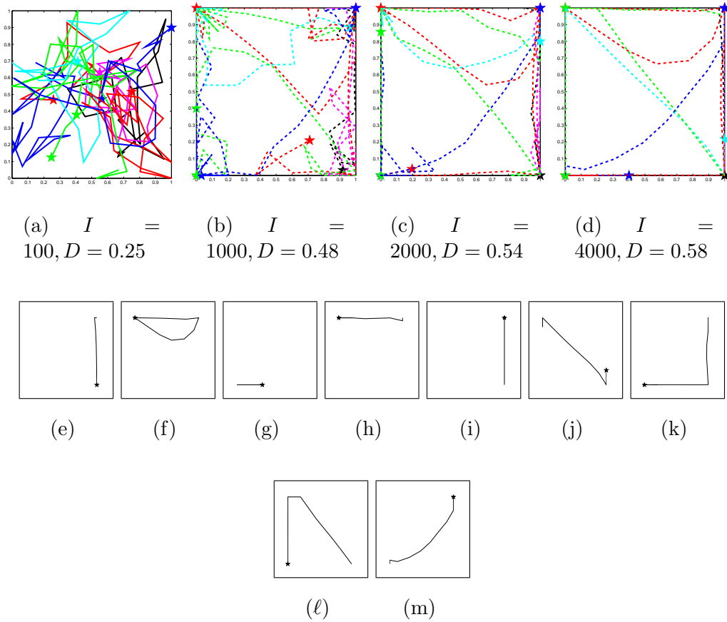
Fig. .8. A repertoire in a 2d acoustic space optimized for distinctiveness. Common parameters: T = 9, P = 20, 2d, S = 0.2, \rho = 0.2, \delta = 0.25 . Figures (a-d) show the configurations at various stages of the hillclimbing process. Figures (e-m) show each of the individual trajectories in figure (d).
