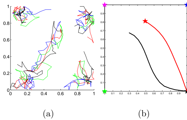
Fig. .12. Comparison of population-based models with the optimization model. Frame (a) shows the (five) trajectories of four agents (from a population of ten). Notice the similarities with the optimized trajectories in frame (b).
