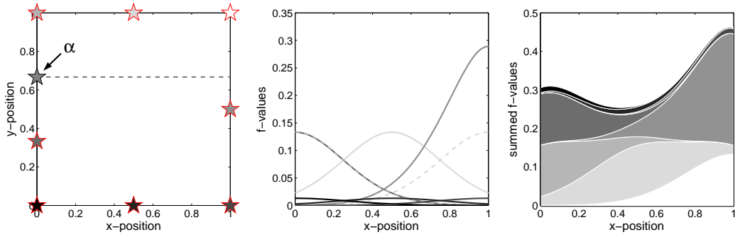
(a) 9 points at a local optimum; we will consider moving one signal \alpha along the horizontal interval.
